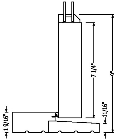
OPTIONAL FLAT BUMPER SILL
