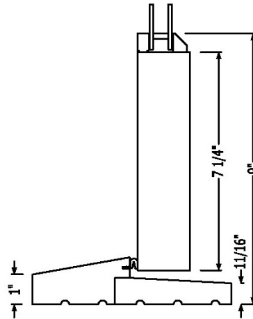
OUTSWING BUMPER SILL
